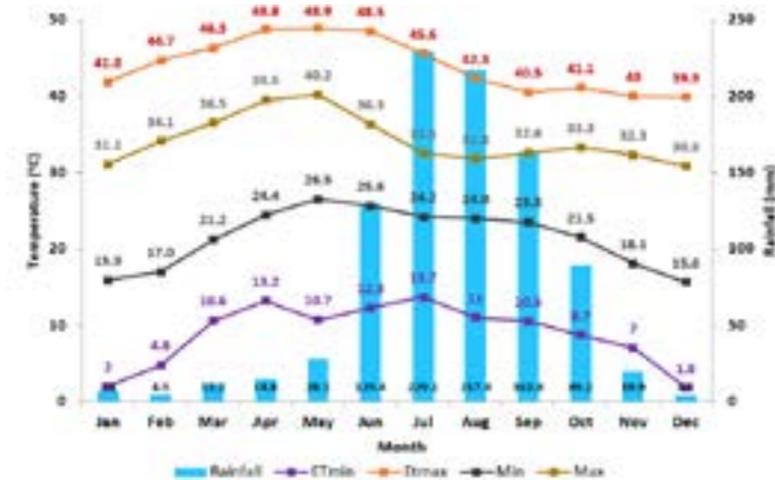
Month wise average Rainfall; Temperature - Extreme Max, Min (24hrs) Avg Max, Avg Min
